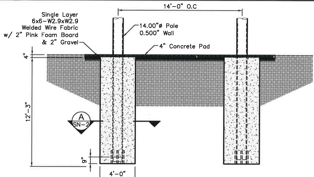
Foundation Elevation SCALE: \frac{3}{8} " = 1'-0"
