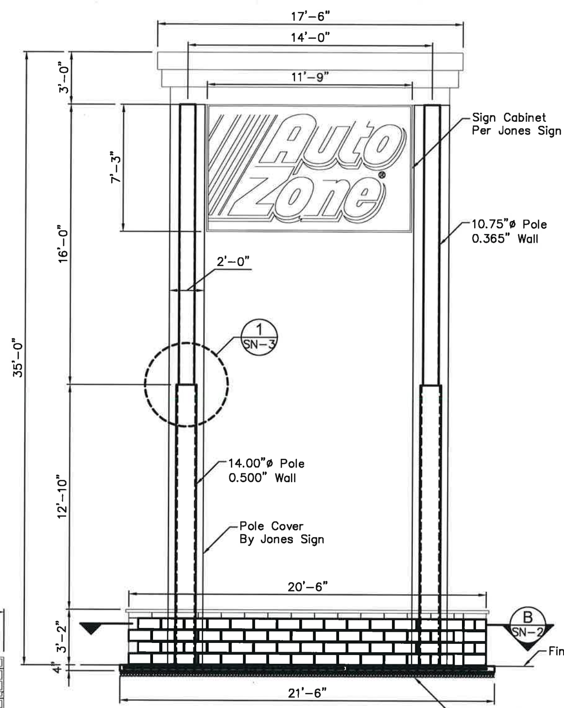
Structure Elevation SCALE: \frac{3}{8} " = 1'-0"
