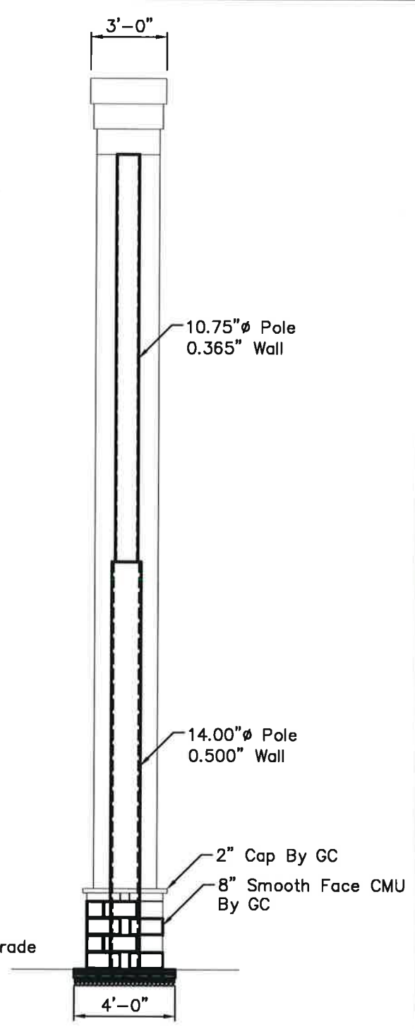
Structure Profile SCALE: \frac{3}{8} " = 1'-0"
